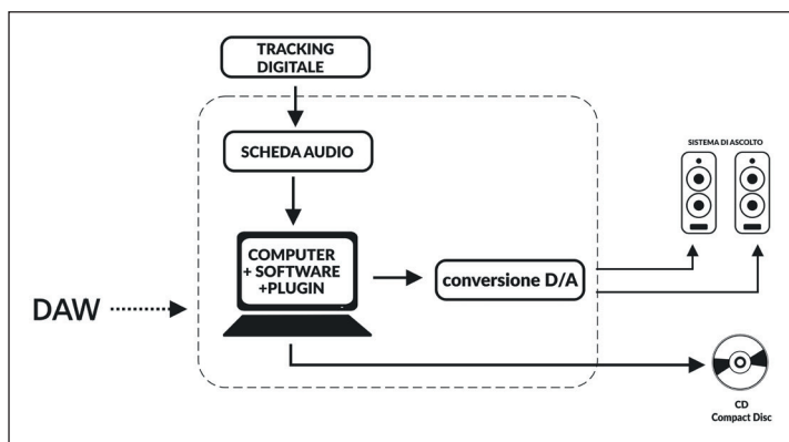
fig. 1.4 Mixing ITB
