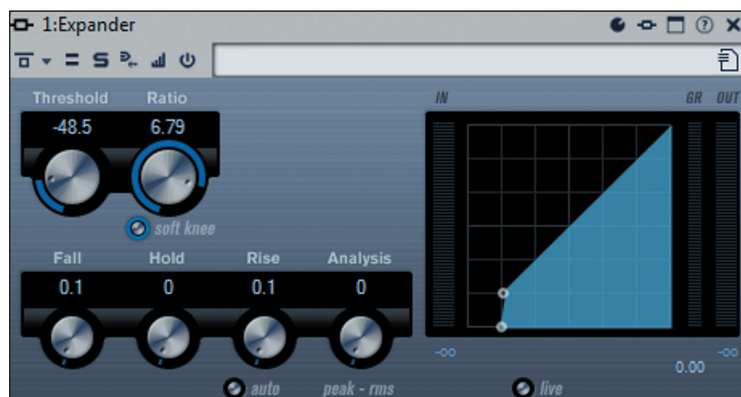
fig. 9.2 Expander per noise reduction
