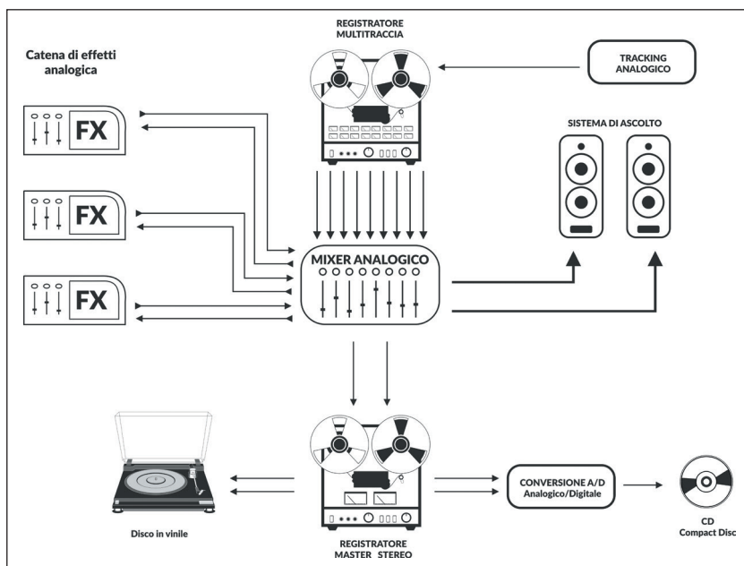
fig.1.3 Mixing OTB
