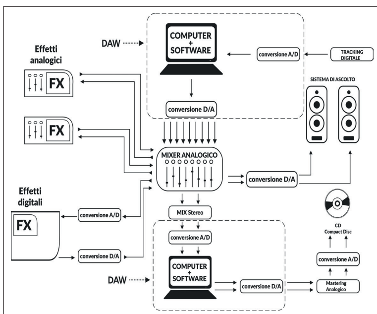
fig. 1.5 Mixing ibrido
